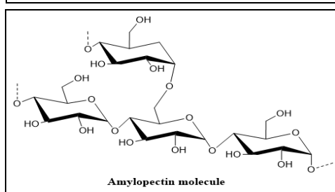
Structure 3: Starch
