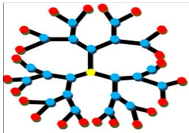
Figure 8: Show Dendrimer
