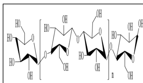
Structure 2: Cellulose
