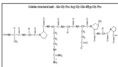
Structure 1: Gelatin
